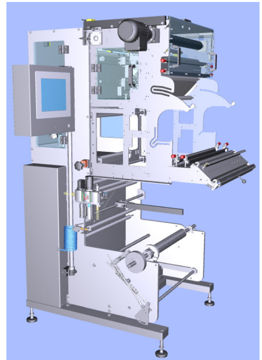
ROVEMA Stabilo Seal® stand-alone unit
