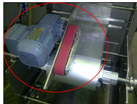
motor-driven unwind device
