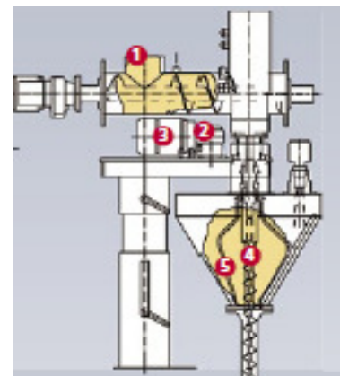
View Auger Dosing (Example)
